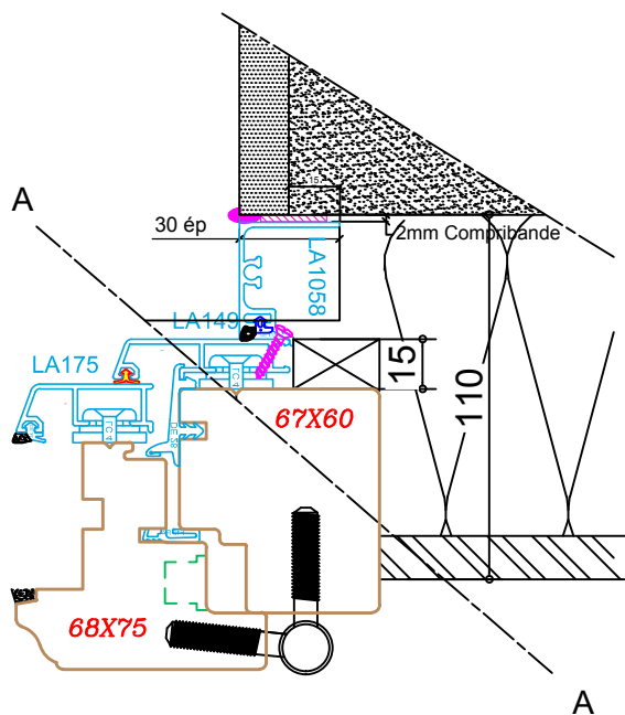
Tapée standard
