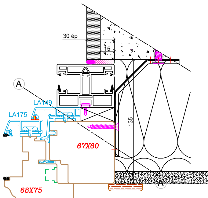
Coulisse standard
