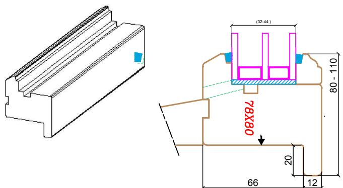
DORMANT "RENOVATION"
