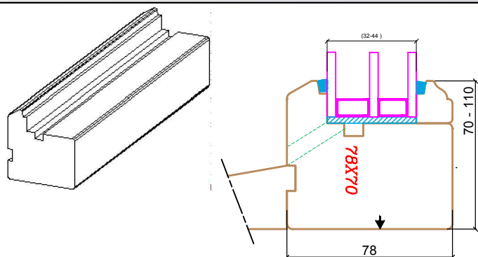
DORMANT "STANDARD"
