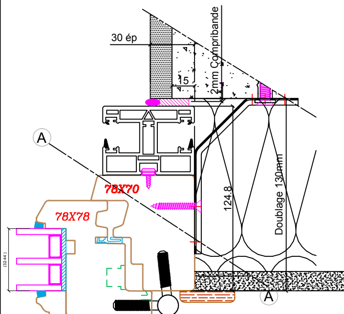
Coulisse standard
