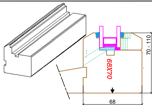
DORMANT "STANDARD"
