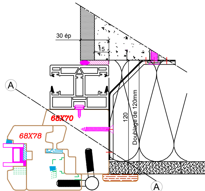
Coulisse standard
