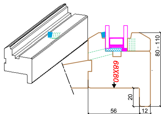
DORMANT "RENOVATION"
